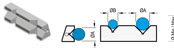
Piastra ganaschia intercambiabile prismatica a pettine Prismatic comb interchangeable jaw plate
